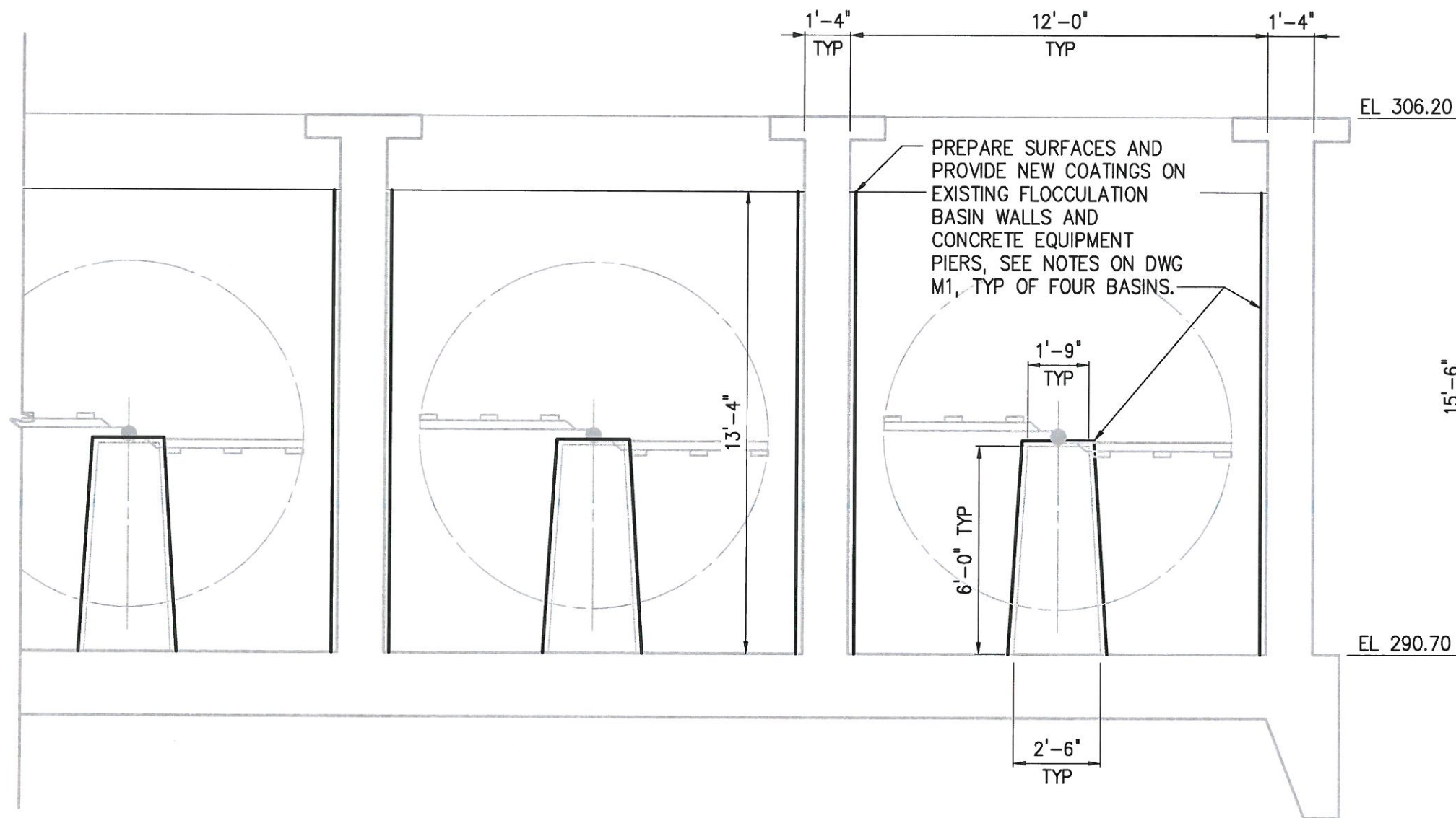
SECTION B-B 1/4" = 1'-0"
