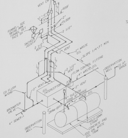
OIL INTERCEPTOR PIPING DIAGRAM NO SCALE
