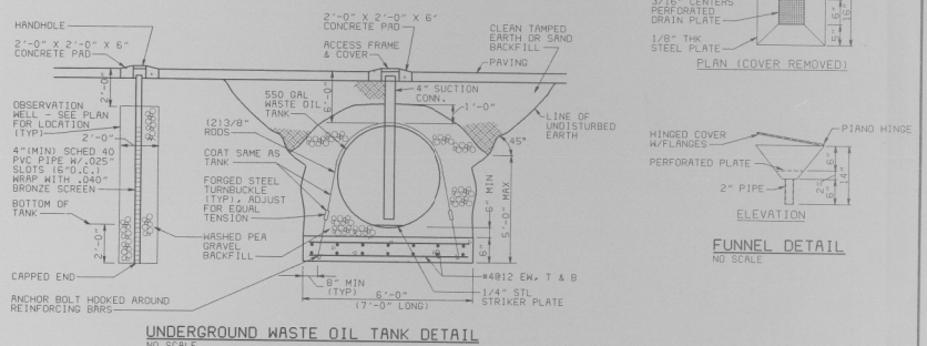
UNDERGROUND WASTE OIL TANK DETAIL NO SCALE
