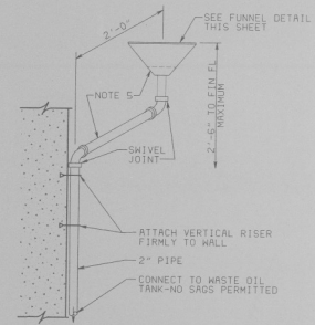
SWING ARM FUNNEL DETAIL NO SCALE
