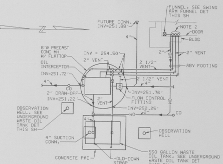
PLAN VIEW-OIL INTERCEPTOR AND WASTE OIL TANK SCALE: 1/4"=1'-0"
