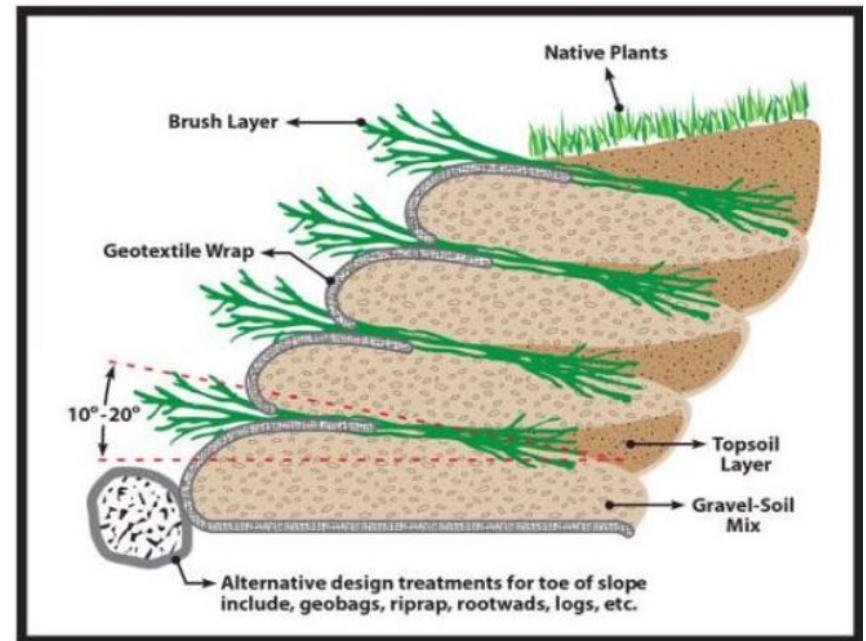
Bioengineering Bank Revetment
